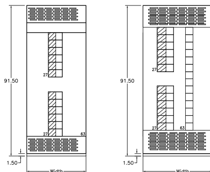
Single Row I-Line Distribution Sections
