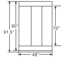
Single Row, 98X 2 Mounting Height MQS Mounting (200A Max)
