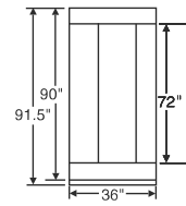
Single Row, 72" Mounting Height QMB Mounting (400A Max.)
